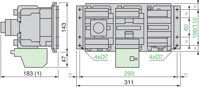
LC3D80 3 x LC1D80
